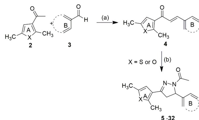
Scheme 1 Reagents and conditions: (a) 5% NaOH, ethanol, rt, 4-5 h, 65-82% (b) NH 2 NH 2 ·H 2 O, CH 3 COOH, reflux, 4-6 h, 75-90%.
