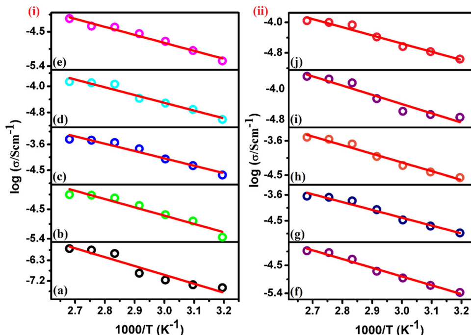
Figure 8 Arrhenius plot for (a) PEO–PVP, and O/Na = (b) 2, (c) 4, (d) 6, (e) 8, (f) 10, (g) 12, (h) 14, (i) 16, (j) 20.
