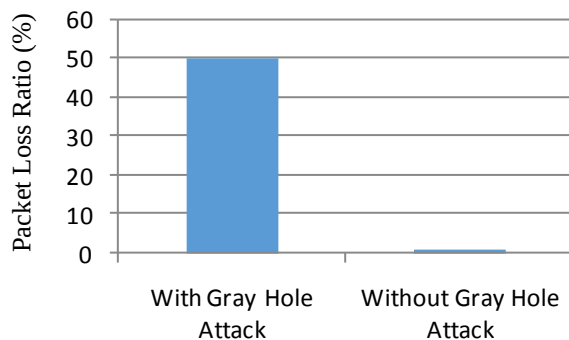
Figure 3 Packet Loss Ratio using Bulksend Application
