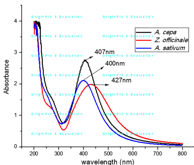
Fig. 2 Absorption spectrum of various plant extracts based on green-synthesized AgNPs (color figure online)
