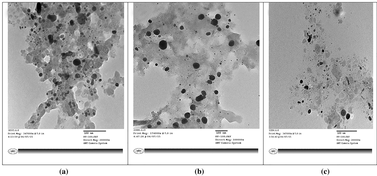
Fig. 4 TEM images of biosynthesized AgNPs and their particle size distribution. a A. cepa , b Z. officinale and c A. sativum
