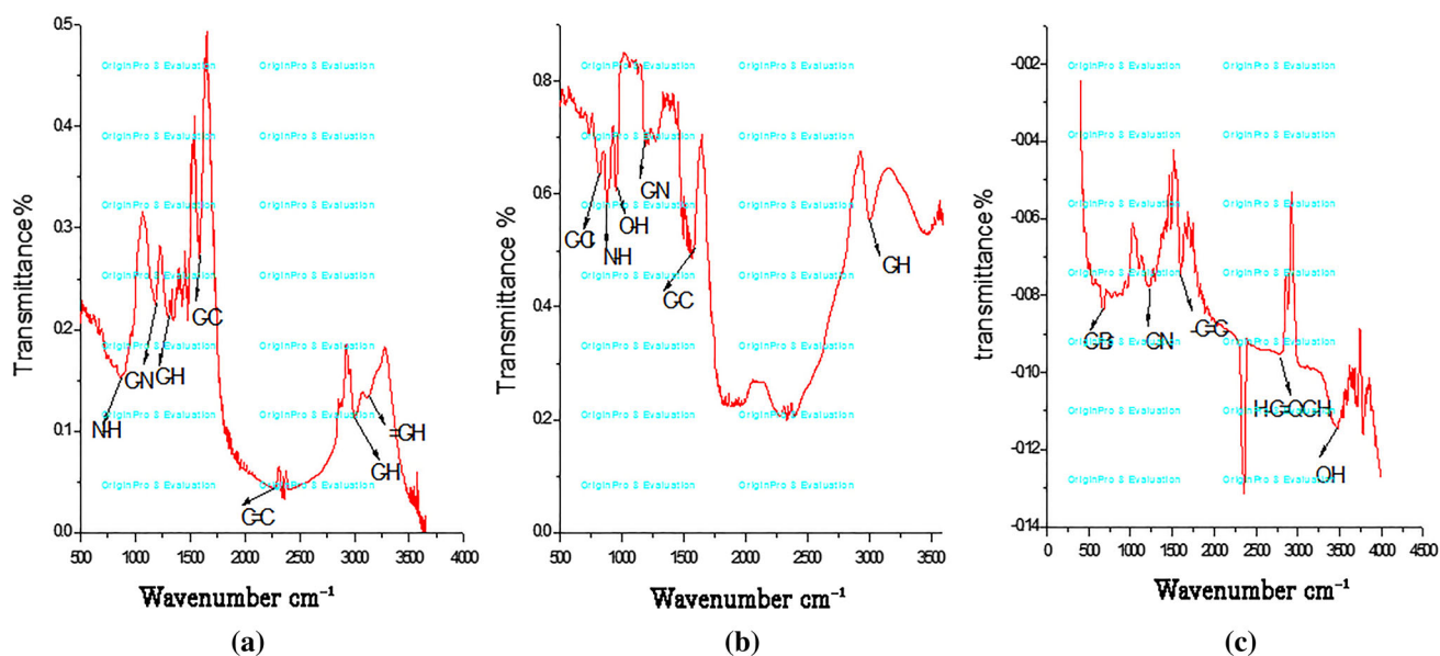
Fig. 3 FTIR analysis of biosynthesized AgNPs a A. cepa , b Z. officinale and c A. sativum
