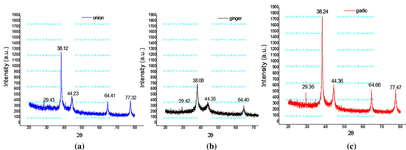
Fig. 6 XRD analyses of AgNPs biosynthesized by plant extracts a A. cepa , b Z. officinale and c A. sativum
