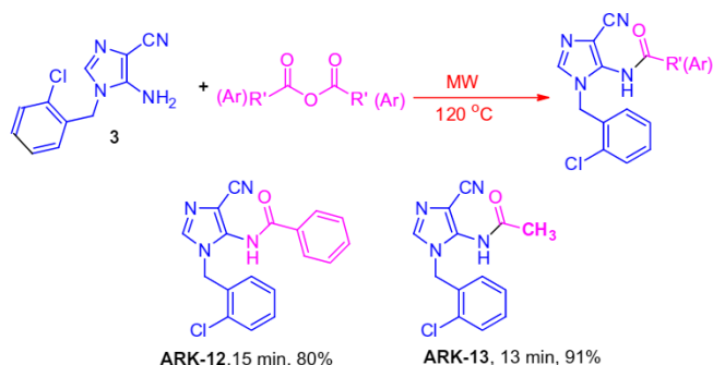
Scheme 3. Synthesis of target compounds (ARK-12-13).
