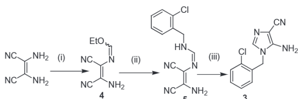
Scheme 1. Reagents and conditions: (i) \text{CH}(\text{OEt})_3 , dry 1,4-dioxane, reflux, 8–10 h; (ii) o -Cl- \text{PhCH}_2\text{NH}_2 , EtOH, aniline hydrochloride (1 mol %), rt, 5–6 h; (iii) 1 M KOH, rt, 7–8 h.
