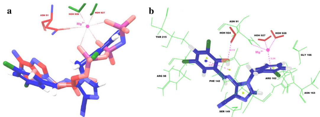
Figure 7. (a) Docking pose of ARK-4 (red) at the binding site of AMPNP (magenta) in ATPase domain of TopoII \alpha ; (b) docking pose of ARK-4 showing the interactions with important amino acid residues in ATPase domain of TopoII \alpha .
