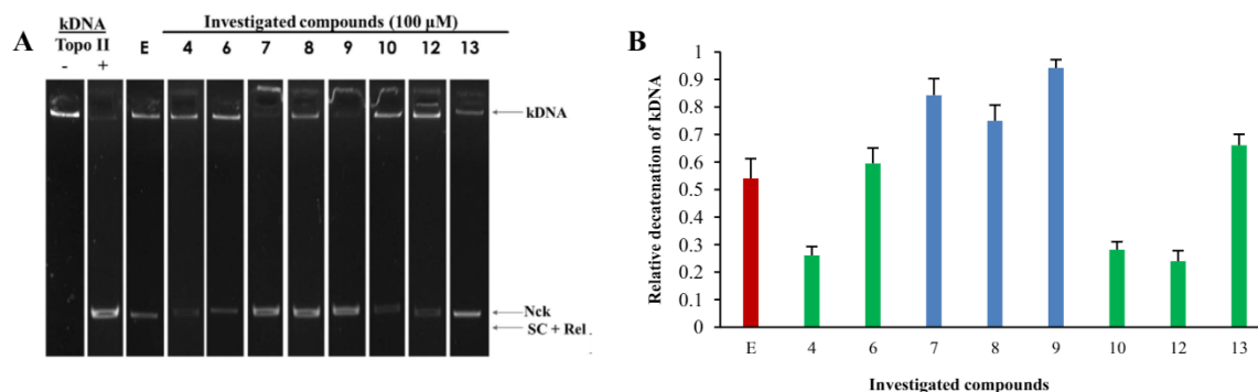
Figure 4. (A) hTopoII \alpha -inhibitory effect of selected ARK series compounds in kDNA decatenation assay. (B) Quantification of product formed in kDNA decatenation assay.
