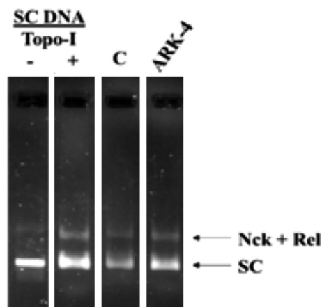
Figure 6. Topoisomerase I relaxation assay: Negatively supercoiled DNA was treated with TopoI in the presence of 100 \mu M camptothecin (C) or ARK-4 , separately.
