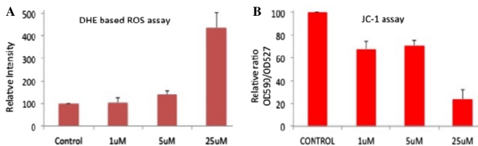
Figure 3. (A) DHE based assay to measure intra-cellular reactive oxygen species (ROS) induced by ARK-4 . (B) JC-1 dye based assay to measure mitochondrial membrane potential altered by ARK-4 .
