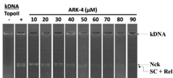
Figure 5. Determination of IC_{50} value of ARK-4 by the inhibition of hTopoII \alpha catalyzed decatenation of kDNA. (Different concentrations of ARK-4 (10–100 \mu M) were used.)
