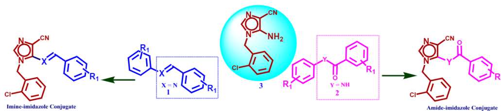
Figure 1. Design of target compounds.
