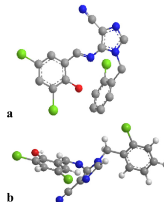
Figure 2. (a) (E)-1-(2-Chlorobenzyl)-5-((3,5-dichloro-2-hydroxybenzylidene)amino)-1H-imidazole-4-carbonitrile, (b) (Z)-1-(2-chlorobenzyl)-5-((3,5-dichloro-2-hydroxybenzylidene)amino)-1H-imidazole-4-carbonitrile.
