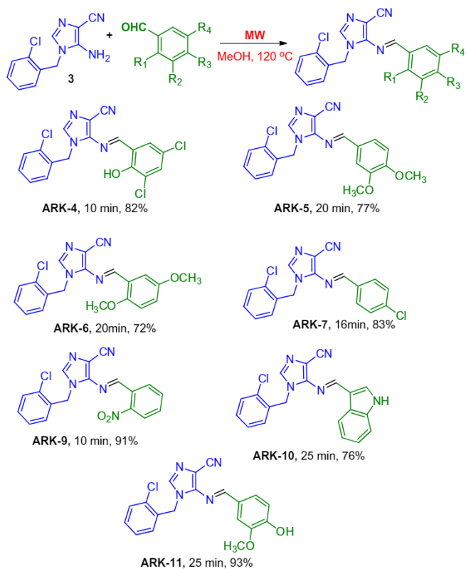
Scheme 2. Synthesis of target compounds (ARK-4-11).
